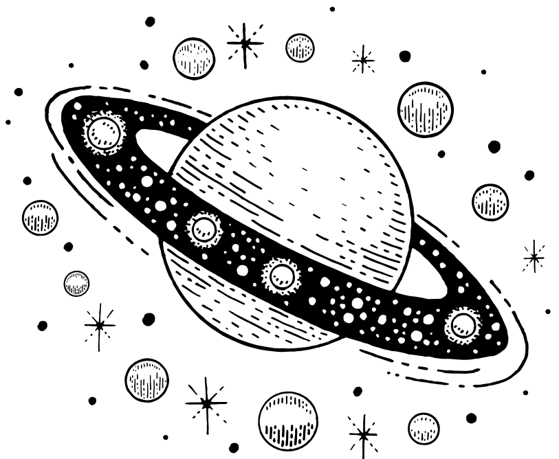
SATURN
